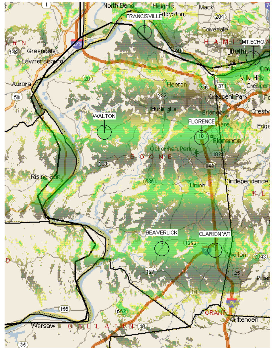
UHF Talk –In Coverage (Law Enforcement)
